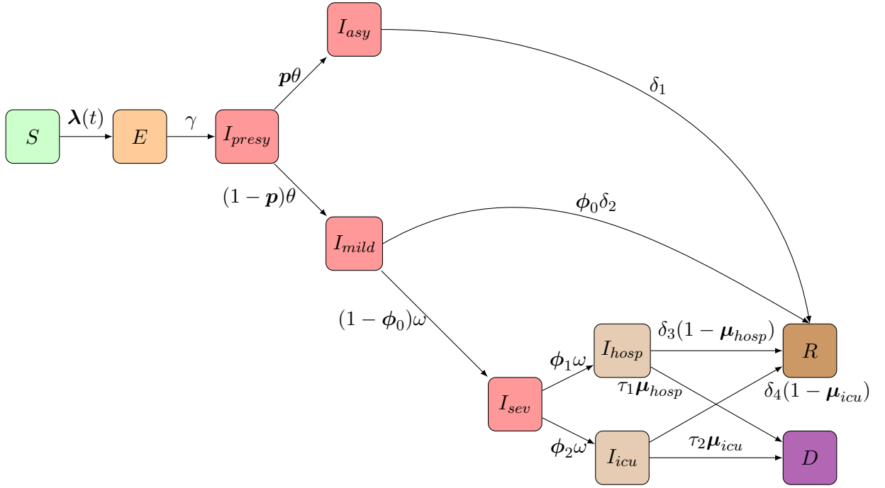
Figure 1: Schematic overview of the flows of individuals in the compartmental model.
